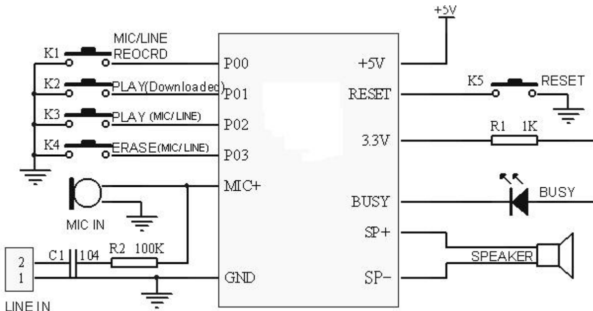
WTV-NAND RECORDING MODULE
